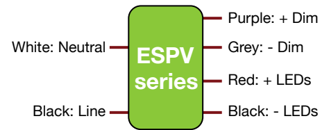
Wiring Diagram
