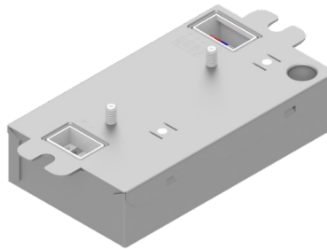
Terminal Blocks (-TN), Metal Case w/ Bottom Studs L 106.7 x W 60.3 x H 25.5 mm (L 4.20 x W 2.37 x H 1.00 in)
