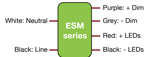
Wiring Diagram
